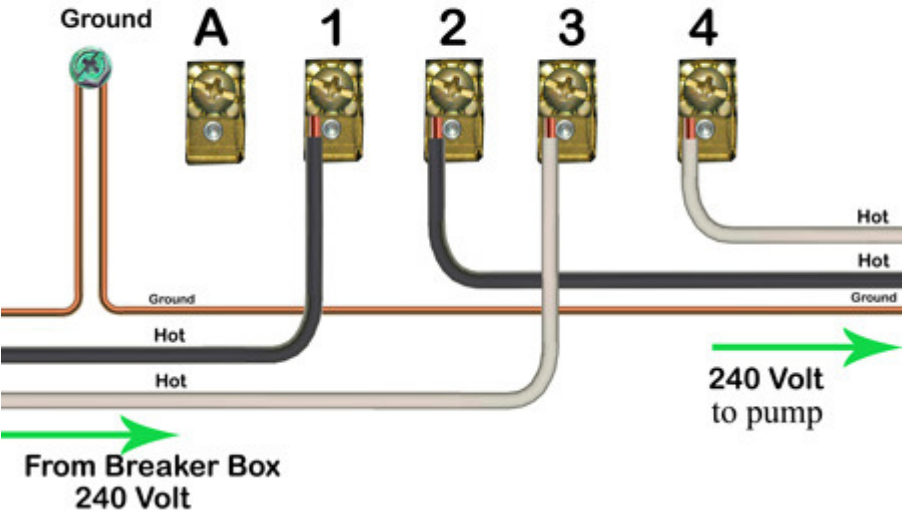
Typical wiring for timer
