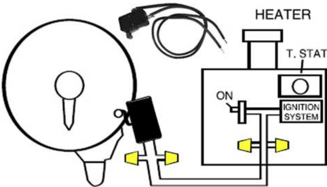
Fireman switch installation
